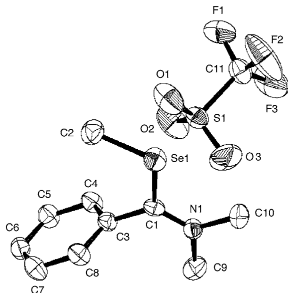
Figure 1. ORTEP drawing of selenoiminium salts 2j . Hydrogen atoms are omitted for clarity. Selected bond lengths (Å): Se1–C1, 1.885(4); Se1–C2, 1.928(4); Se1–C1, 1.280(5); N1–C10, 1.461(5); C1–C3, 1.483(6). Selected torsion angles (deg): Se1–C1–N1–C9, 177.7(3); Se1–C1–N1–C8, 83.0(5); N1–C1–Se1–C2, 166.8(4); C3–C1–N1–C9, 1.7(6).
